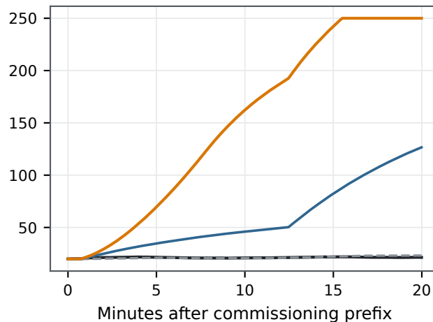
Stator-core temperature (°C)
