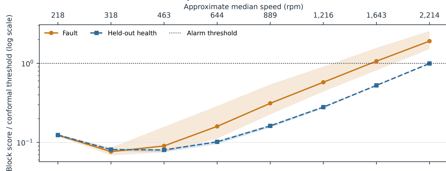
(a) Threshold-normalized anomaly score
