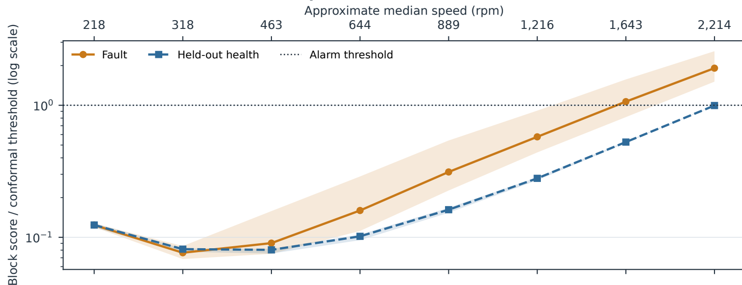
(a) Threshold-normalized anomaly score
