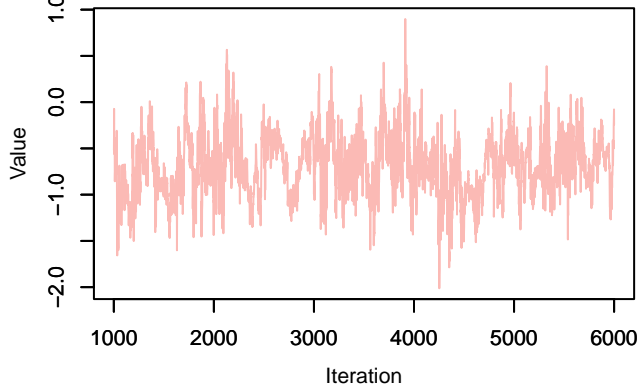
Trace – as.factor(habitat)mixed
