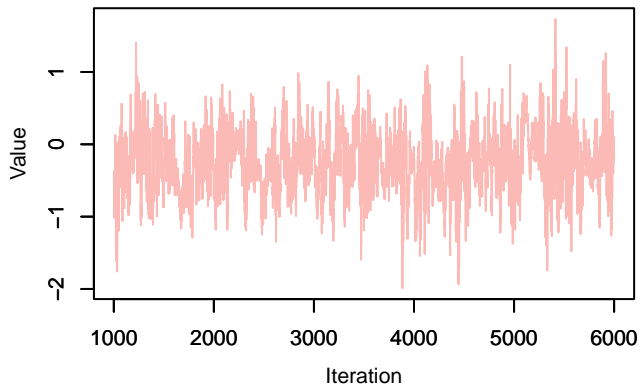
Trace – as.factor(region)North
