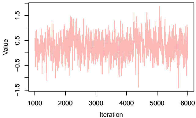
Trace – as.factor(region)South
