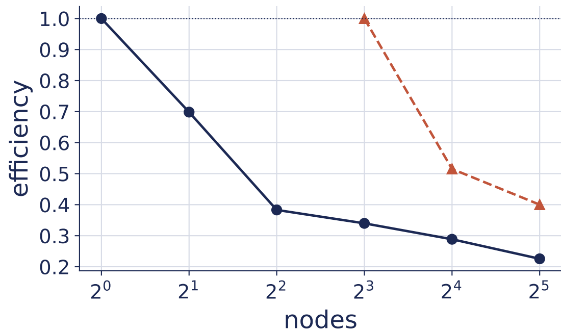
Distributed engine: NUMA-domain vs. node granularity ( \varepsilon = 2^{-16} )
