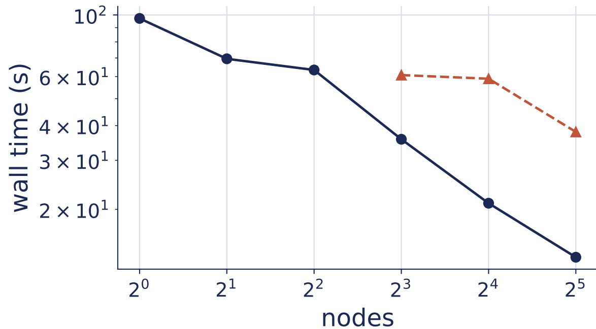
Distributed engine: NUMA-domain vs. node granularity ( \varepsilon = 2^{-16} )
