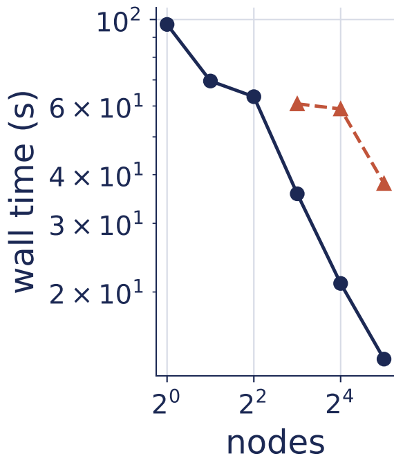
Distributed engine: NUMA-domain vs. node granularity ( \varepsilon = 2^{-16} )
