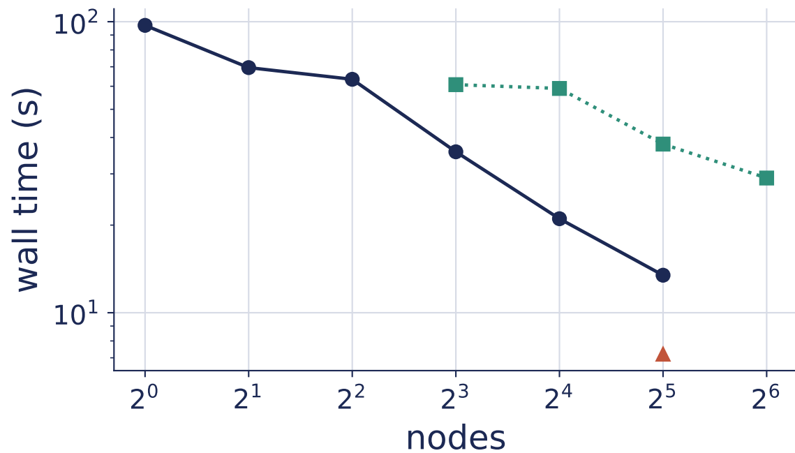
Distributed engine: NUMA-domain vs. node granularity ( \varepsilon = 2^{-16} )
