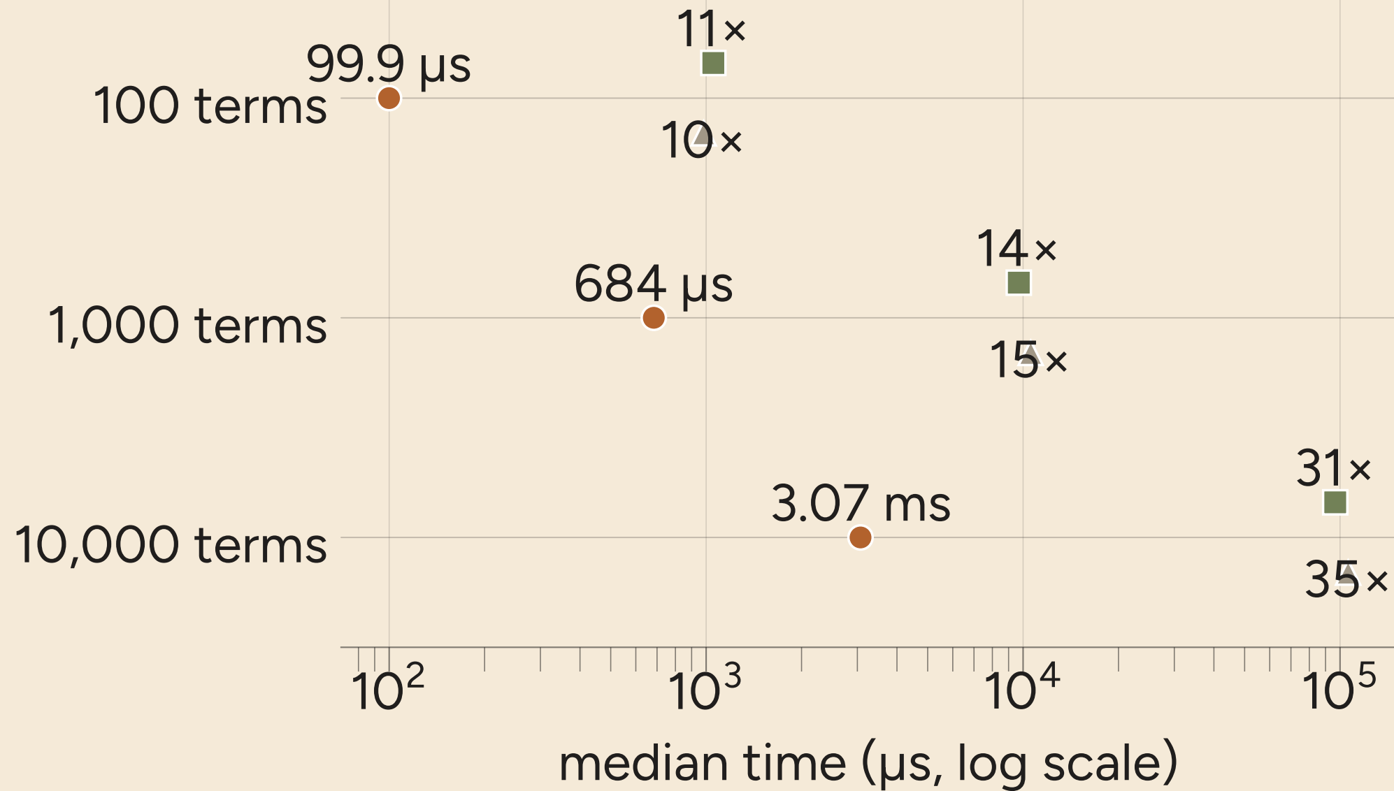
Construct from string terms
