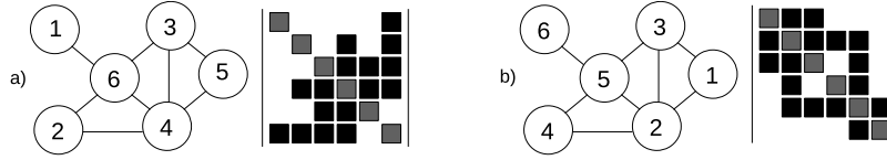
Fig. 1. (a) A graph and its adjacency matrix with the diagonal elements emphasized. (b) The graph after applying a heuristic for bandwidth reduction and the pattern of the corresponding adjacency matrix.
