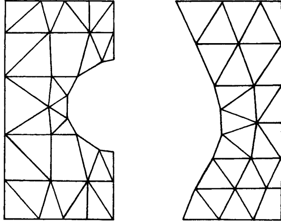
Figure 8.1 Examples of domain discretization by triangular elements.
