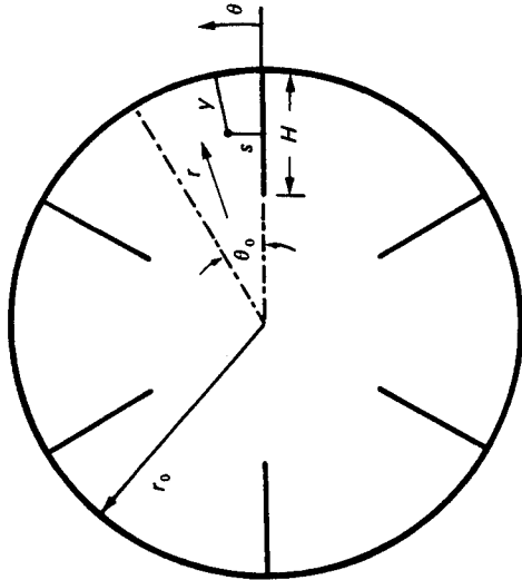
Figure 9.8 Cross-sectional geometry of an internally finned tube [from Patankar, Ivanović, and Sparrow (1979)].
