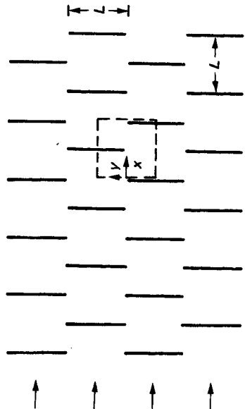
Figure 9.17 Transverse-plate array [from Patankar, Liu, and Sparrow (1977)].
