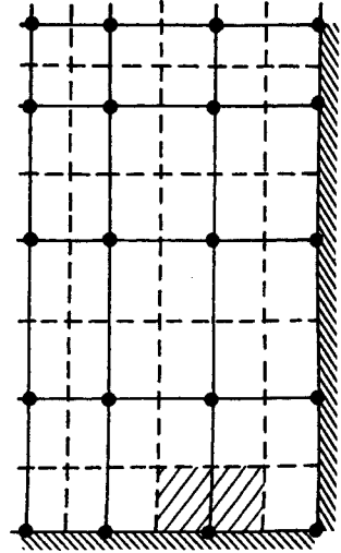
Figure 4.13 Boundary control volumes in Practice A.
