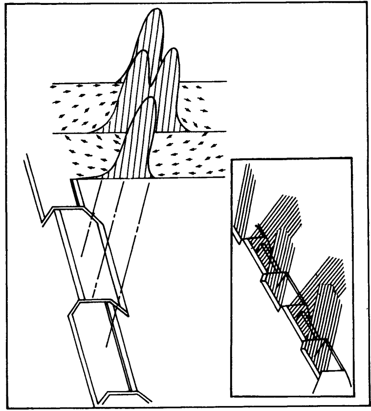
Figure 9.13 Geometry and the flow field of a hypermixing jet [from DeJooode and Patankar (1978)].
