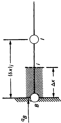
Figure 4.4 Half control volume near the boundary.
