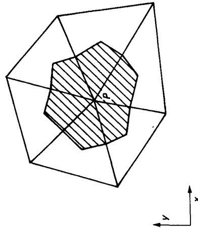
Figure 8.2 Control volume for the triangular grid.
