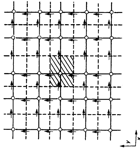
Figure 6.6 Staggered locations for u and v . \rightarrow = u ; \uparrow = v ; \circ = other variables.
