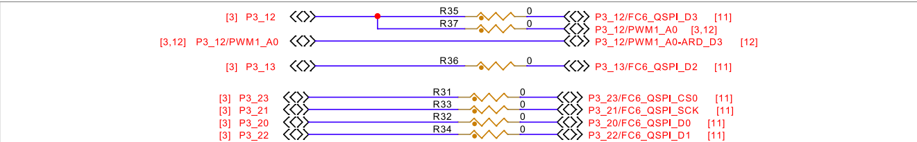
Figure 14. Isolation resistors for flash memory
