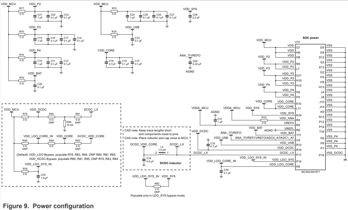
Figure 9. Power configuration
