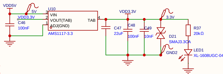
LDO转3.3V电源
