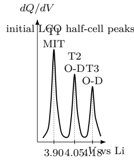
Figure 9: LCO equilibrium dQ/dV peak candidates from the same Q_j \xi_{eq}(1 - \xi_{eq})/w_j formula. T1 near 3.90 V is the MIT peak; T2/T3 near 4.05 and 4.17–4.20 V are order–disorder peaks. The drawing is schematic: Q_j , w_j , and U_j shifts are fit parameters.
