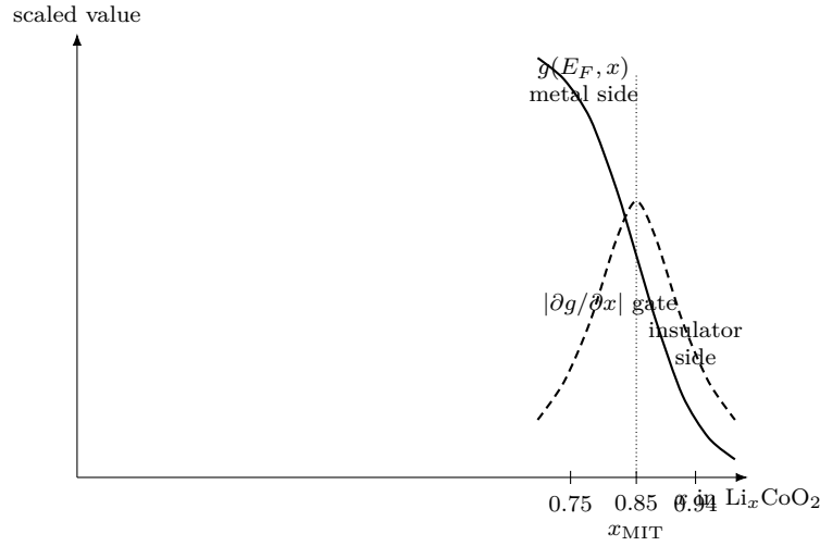
Figure 8: LCO electronic entropy gate. Solid curve is the MIT logistic density of states in eq. (1.37); dashed curve is the localized derivative magnitude that enters \Delta S_e in eq. (1.36). Labels are model-initial values, not fixed material constants.
