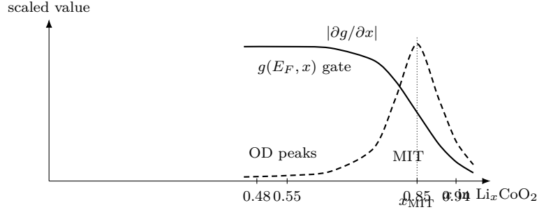
Figure 8: LCO electronic gate (new). Solid line: g(E_F, x) model in Eq. (1.37). Dashed line: local electronic entropy contribution proportional to |\partial g/\partial x| in Eq. (1.36). Labels are model anchors, not fitted results.
