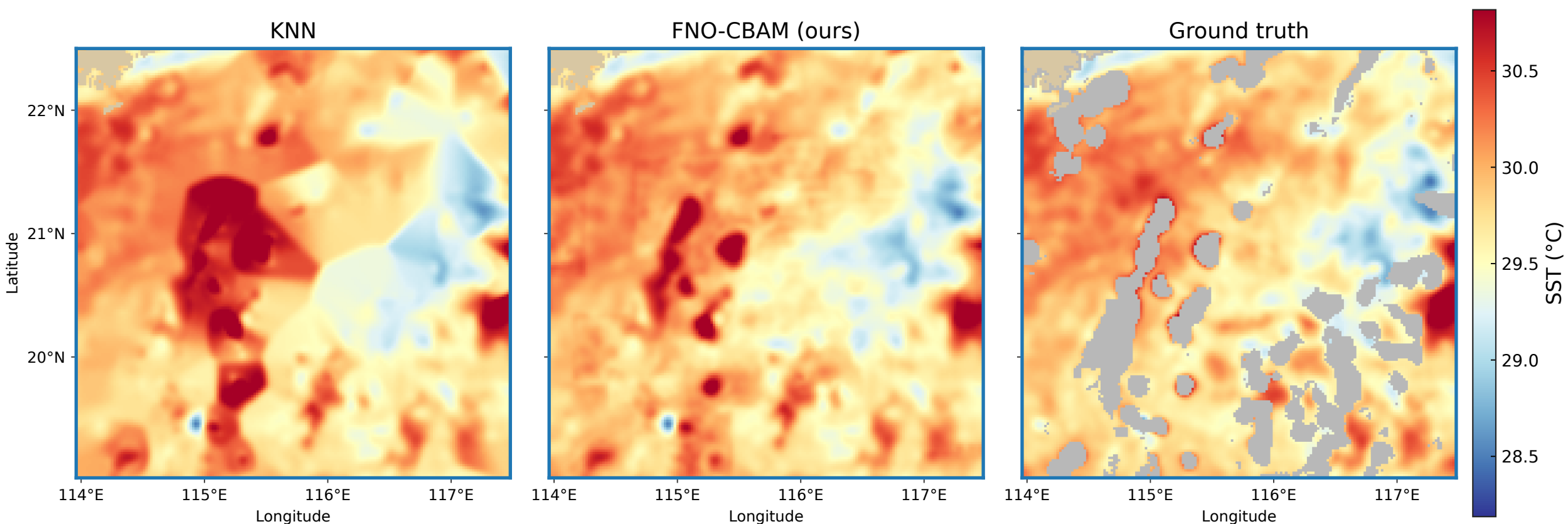
Zoom detail of the boxed region in Fig. 4 (19.0-22.5°N, 114.0-117.5°E)
