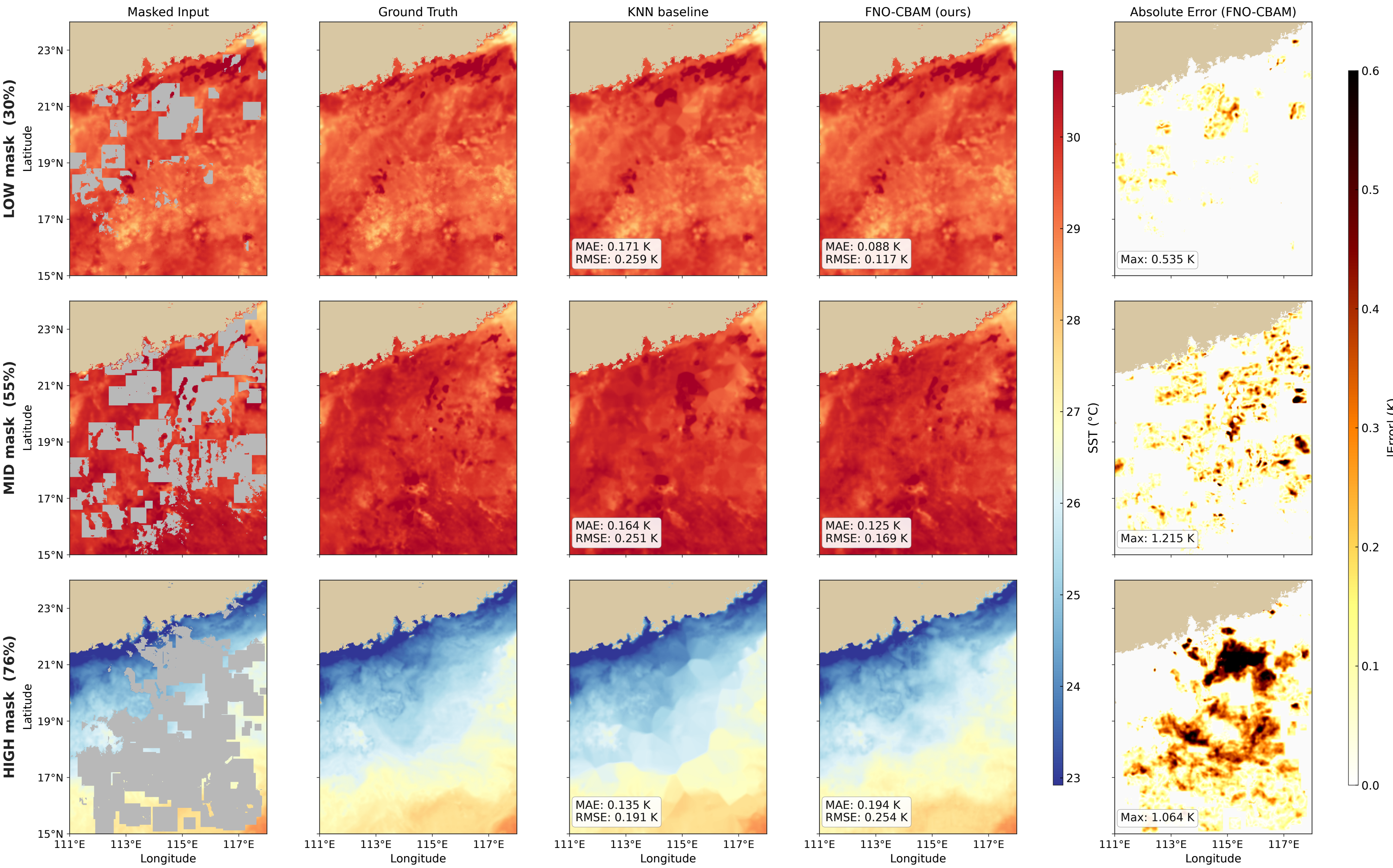
Reconstruction comparison: KNN baseline vs FNO-CBAM (low / mid / high masking)
