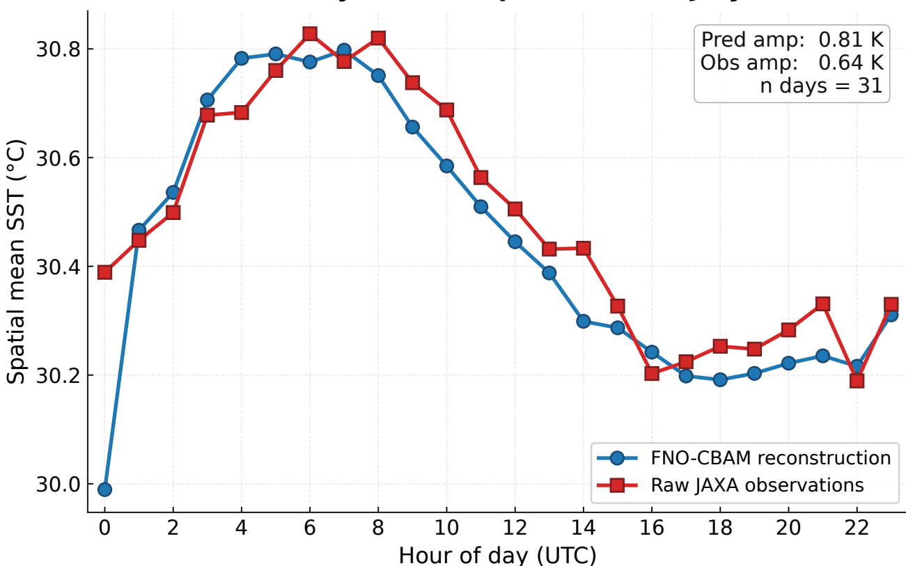
(c) Diurnal cycle (SCS spatial mean, July 2024)
