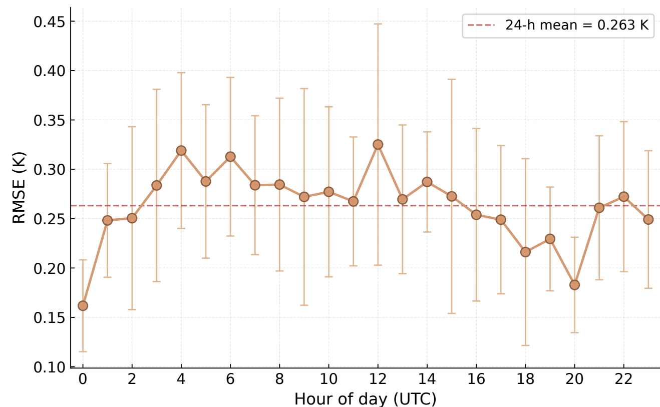
(b) Per-hour RMSE
