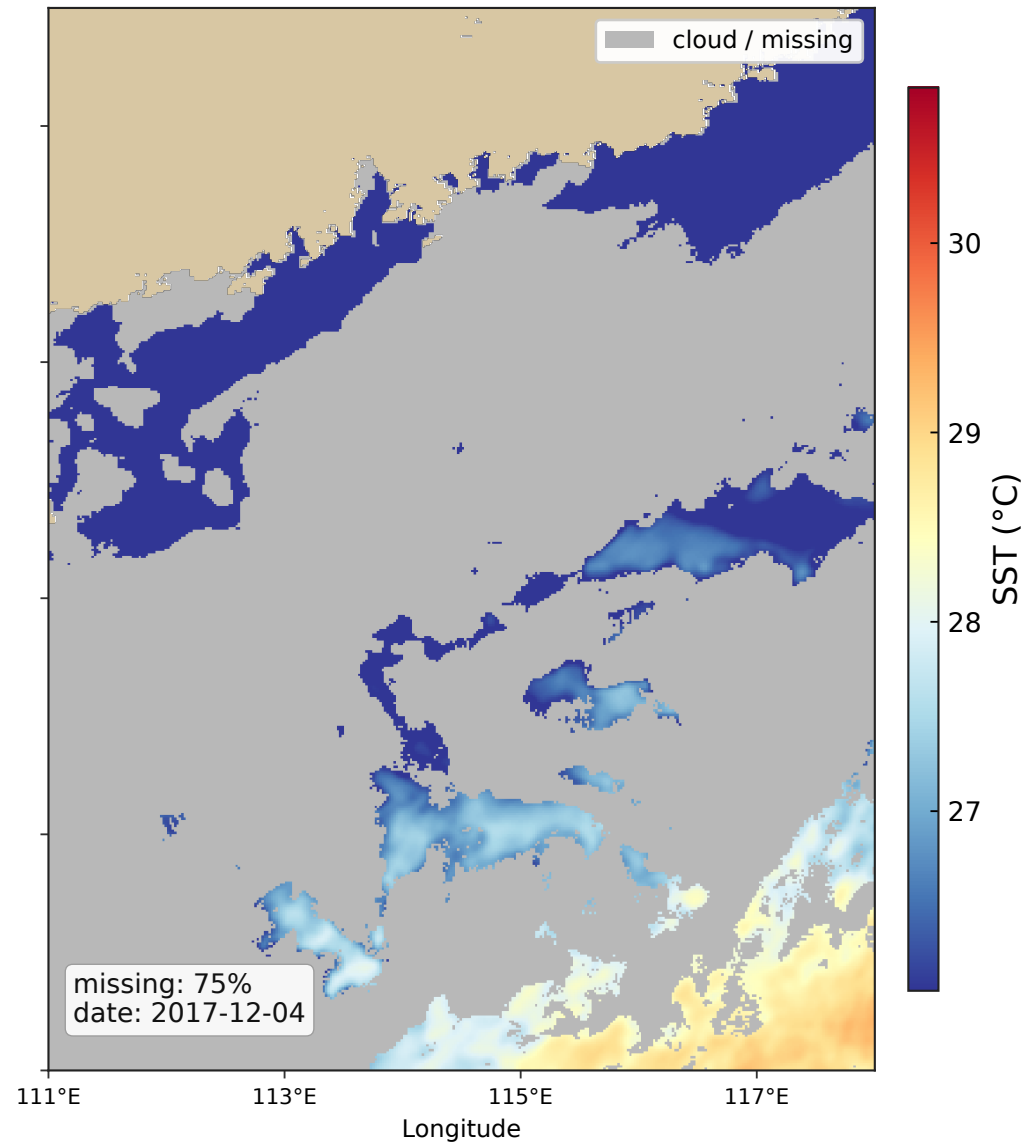
(b) Raw Himawari-8 SST — cloud gaps
