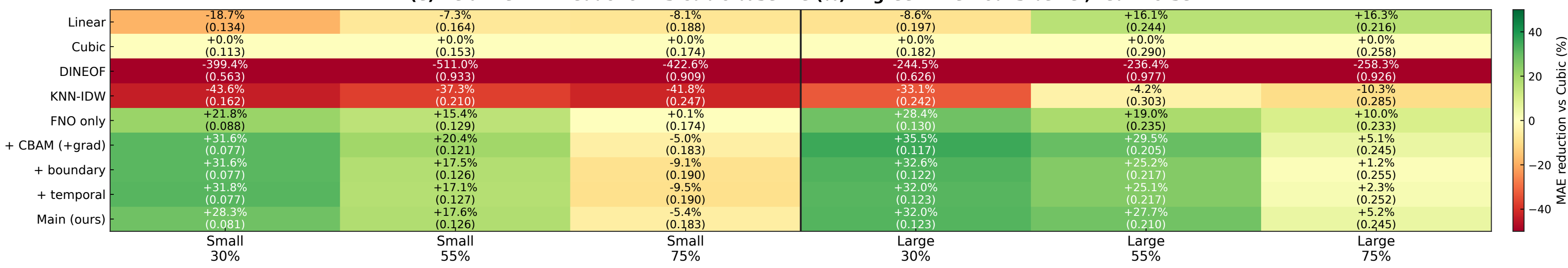
(e) Relative MAE reduction vs Cubic baseline (%) — green: method is better, red: worse
