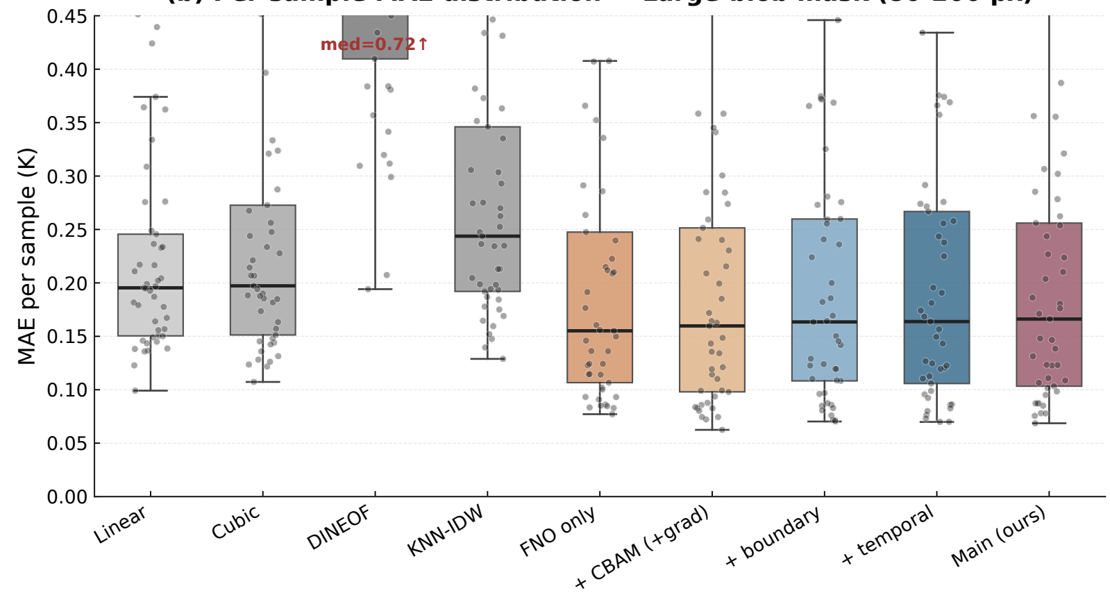
(b) Per-sample MAE distribution — Large-blob mask (80-200 px)
