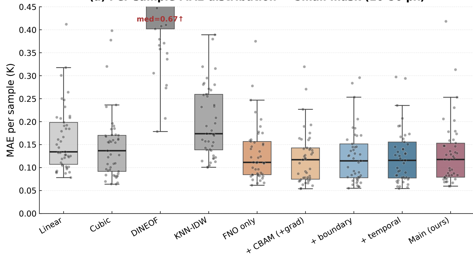
(a) Per-sample MAE distribution — Small mask (10-50 px)
