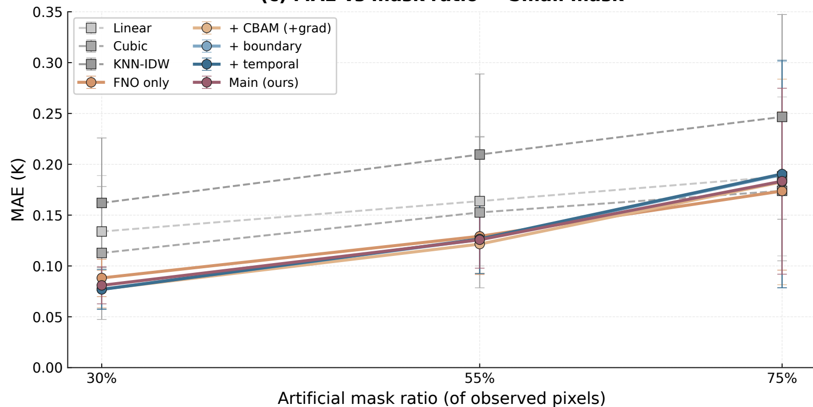
(c) MAE vs mask ratio — Small mask
