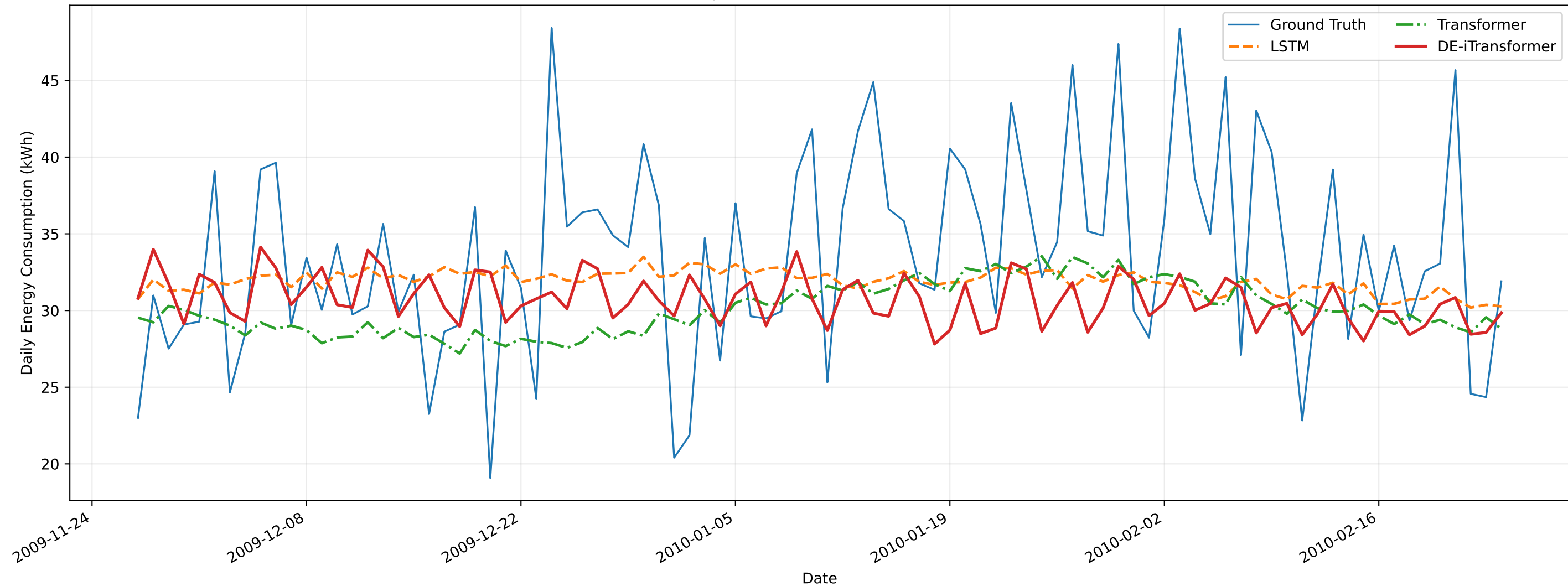
Forecast Comparison of Three Models (Horizon=90)
