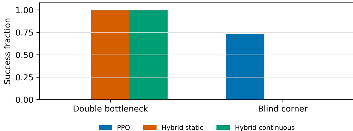
Observed cross-cell inversion (release cells, n=30 each)
