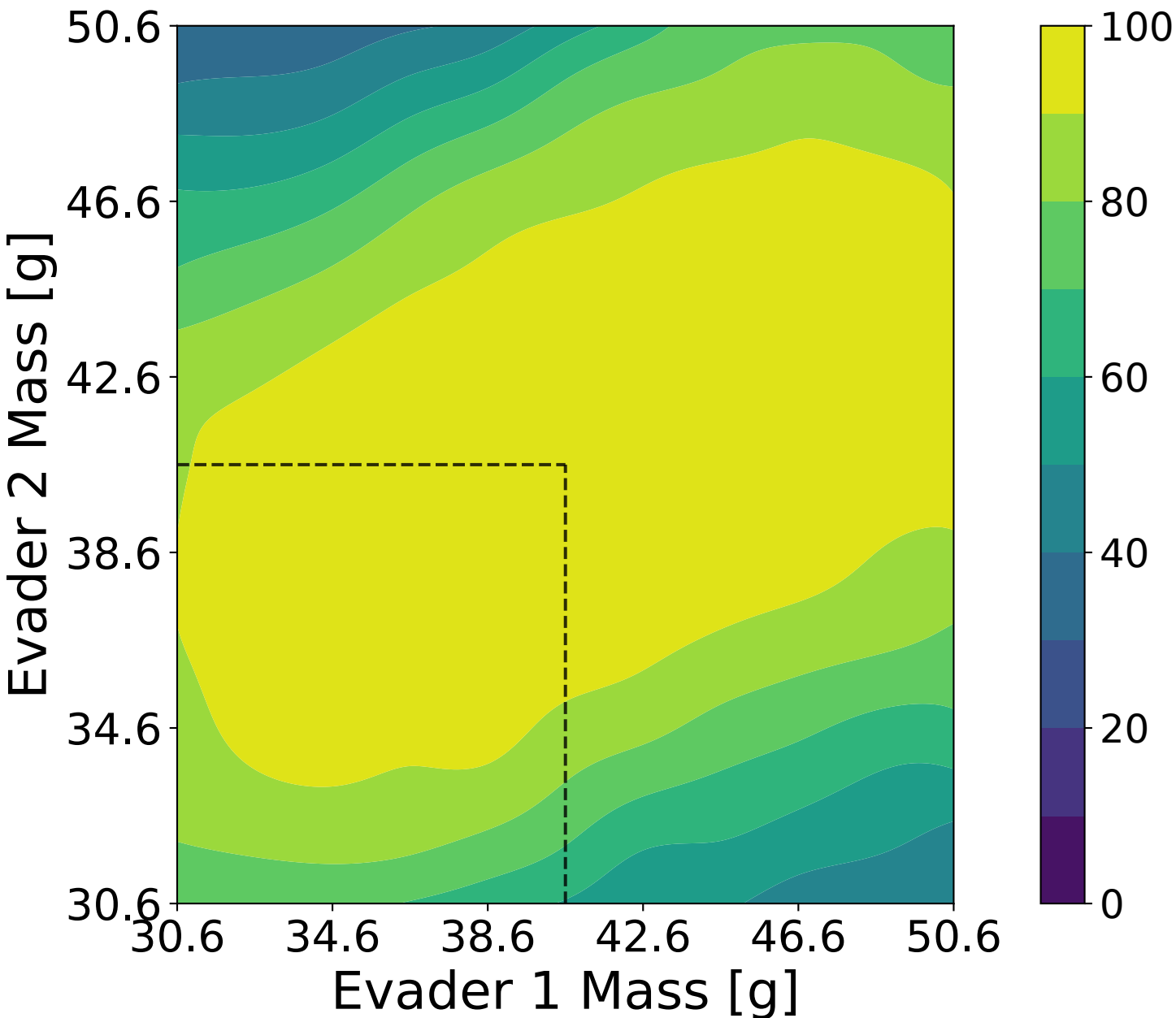
MA-ACMPC: Evader Win Rate
