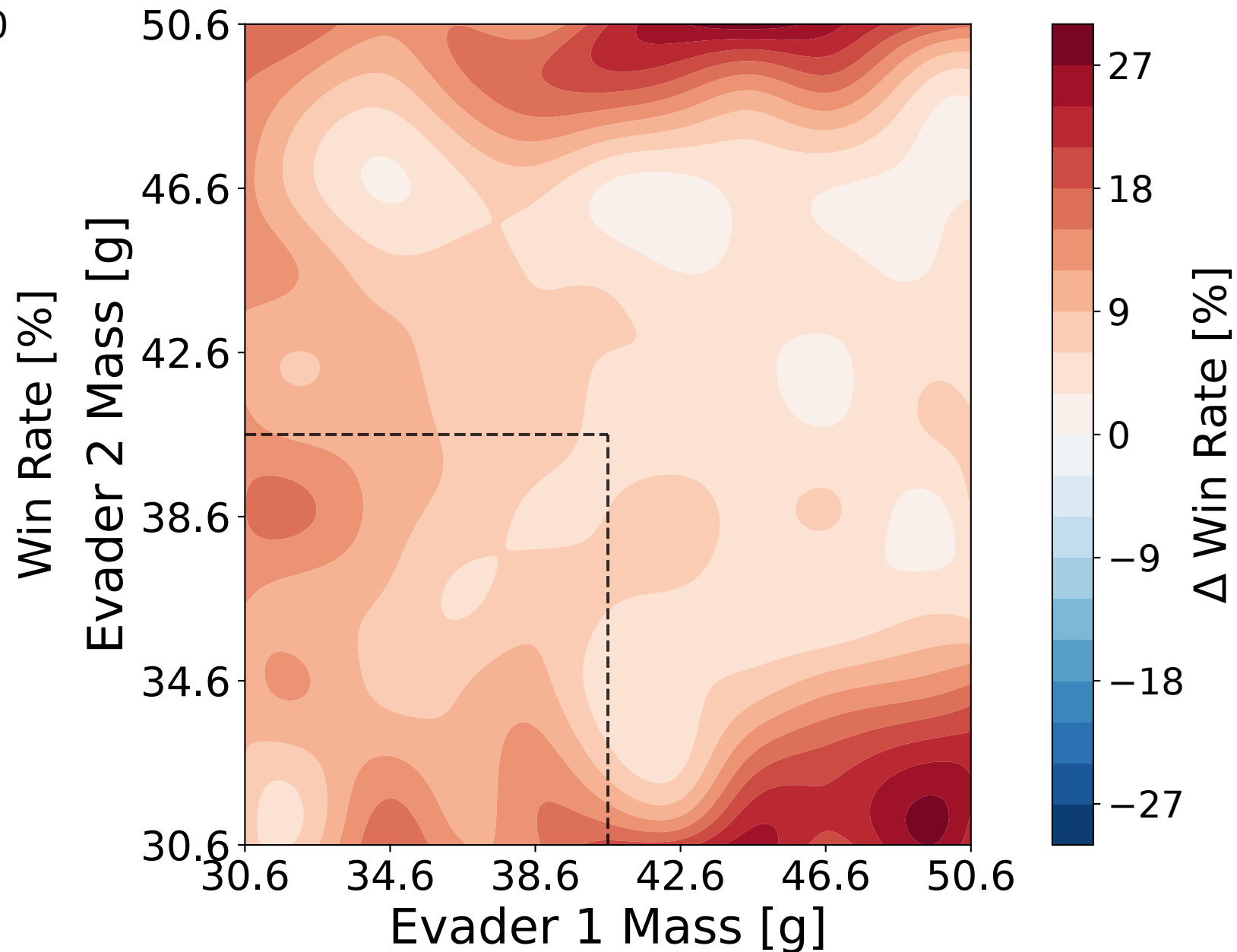
Delta (MA-ACMPC - MLP)
