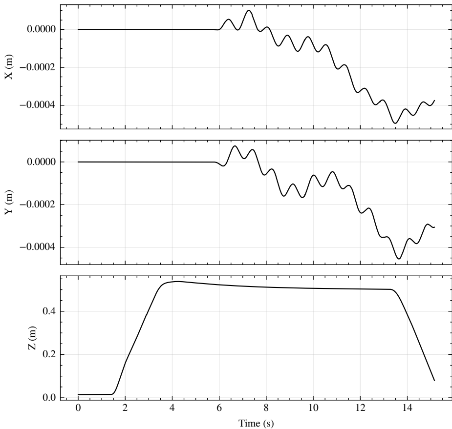
CrazySim State Estimate — Position
