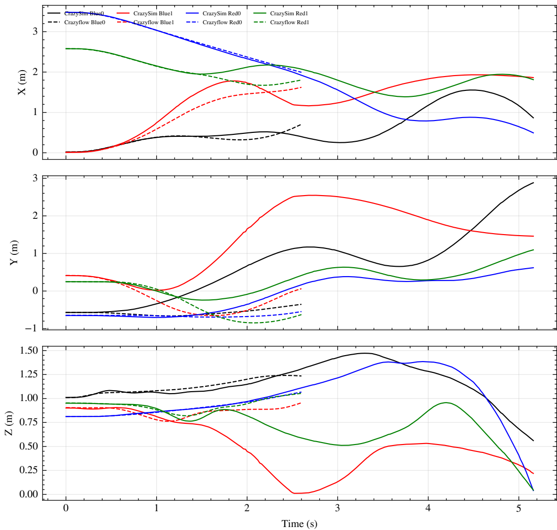
CrazySim vs Crazyflow: MAPE Trajectory Comparison
