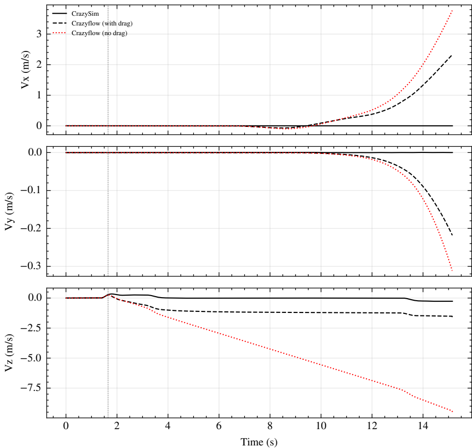
Open-Loop Replay: Velocity Comparison (mass=0.0406 kg)
