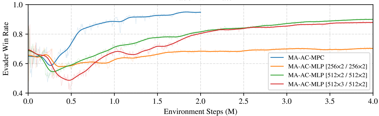
Evader Win Rate
