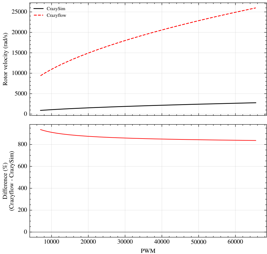
Rotor Velocity: CrazySim vs Crazyflow (cf2x\_T350)
