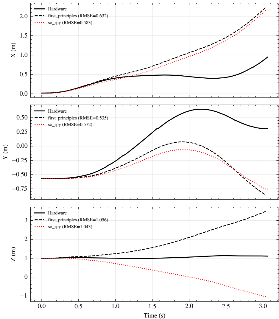
blue_1 — Position: HW vs Sim (mass=0.0406 kg)
