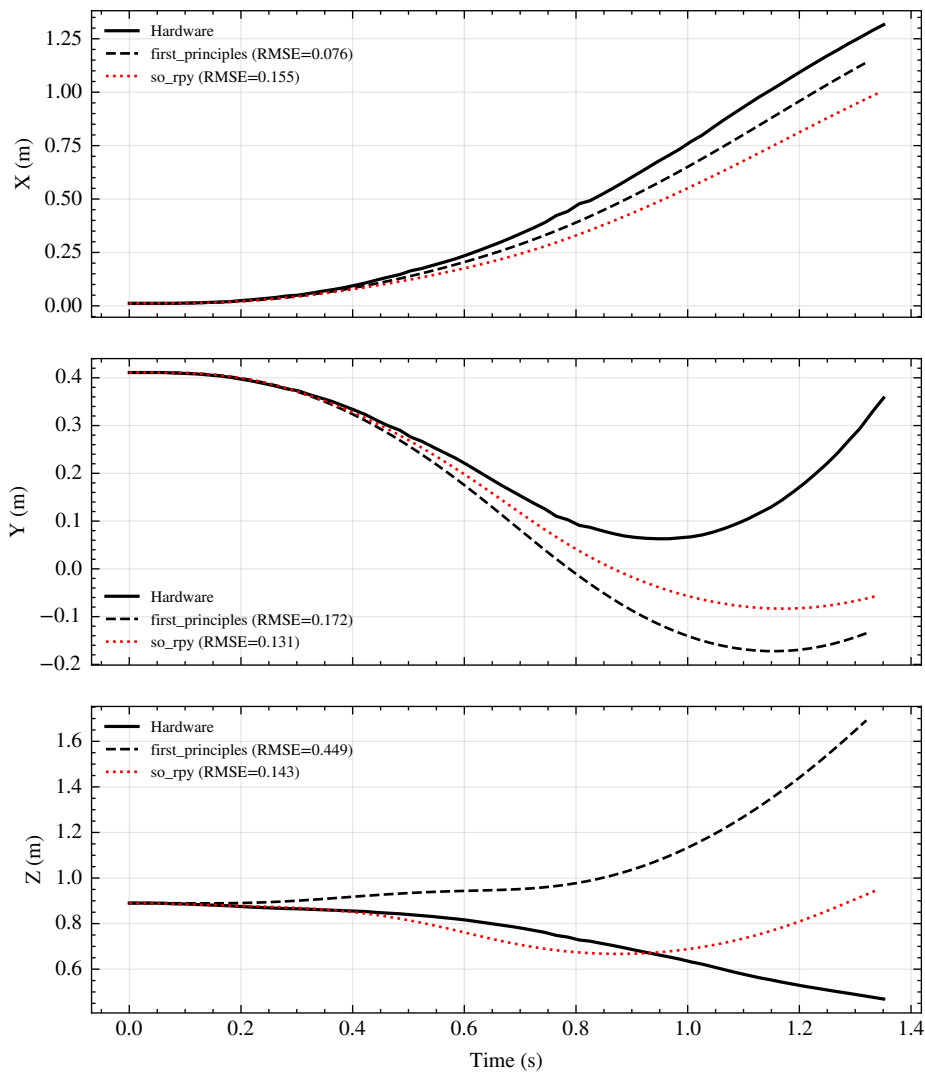
blue_2 — Position: HW vs Sim (mass=0.0406 kg)
