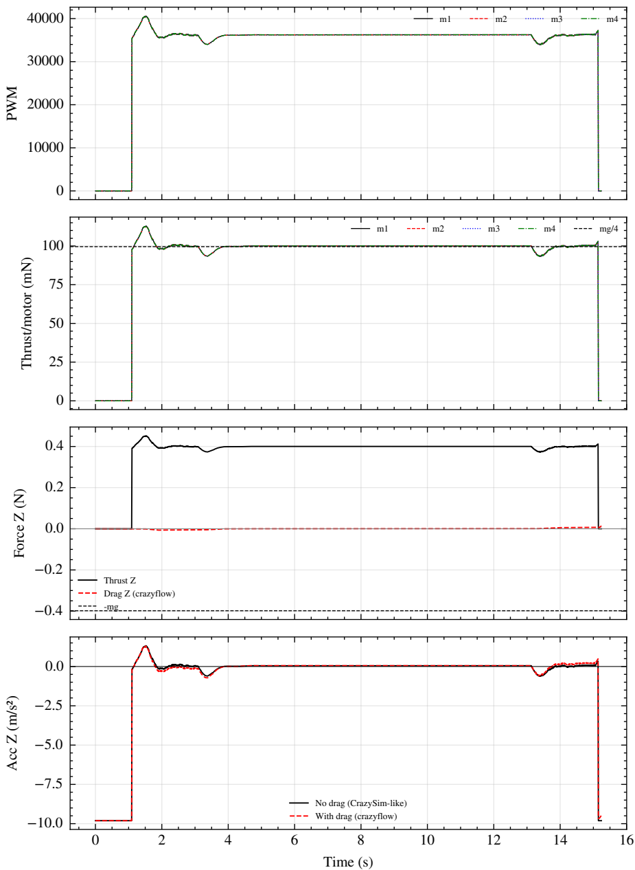
Force Analysis: CrazySim Motor Rates \rightarrow Crazyflow Physics (mass=0.0406 kg)
