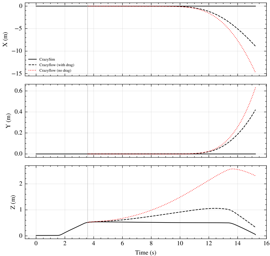
Open-Loop Replay: CrazySim vs Crazyflow (mass=0.0406 kg)
