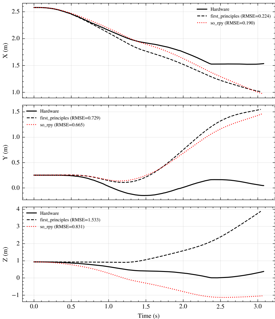
red_2 — Position: HW vs Sim (mass=0.0406 kg)
