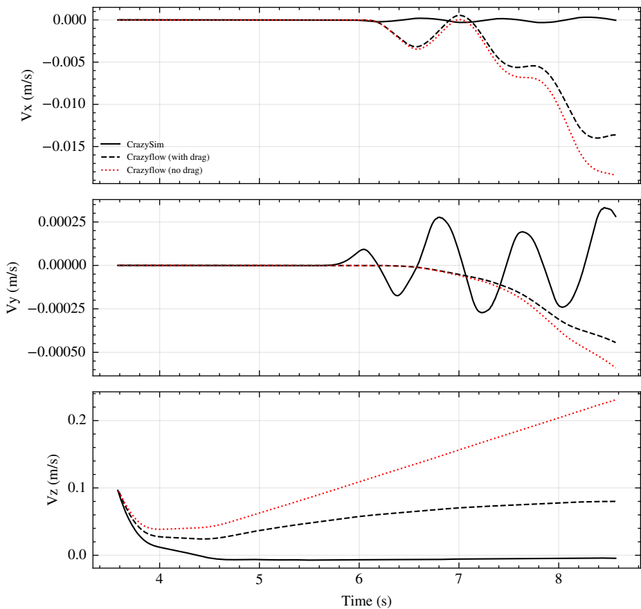
Velocity Comparison — First 5s (mass=0.0406 kg)
