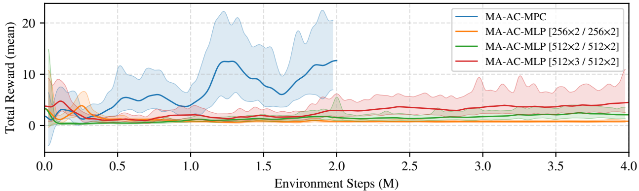
Total Reward (Mean)
