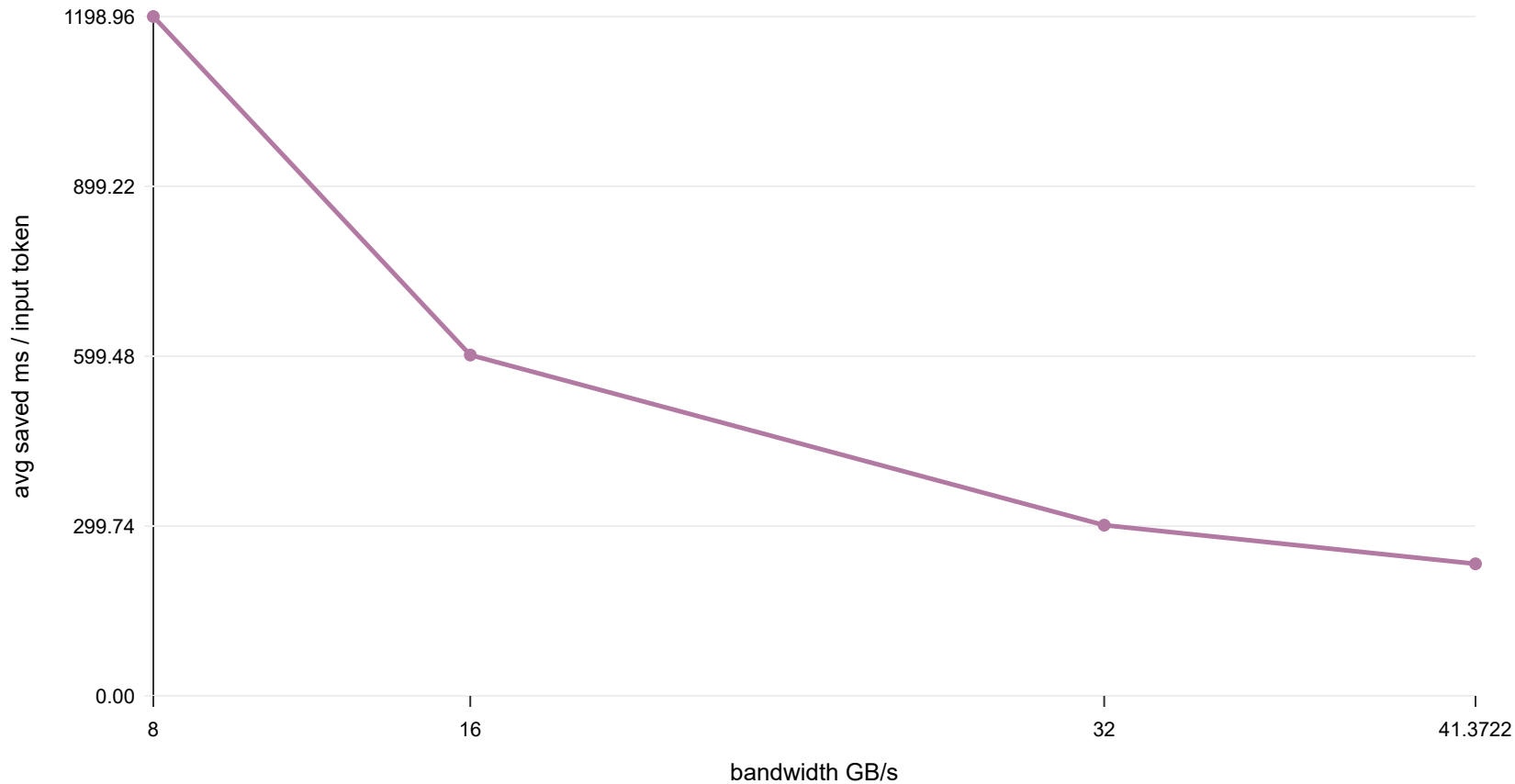
WREC-H2 Saved Stall vs Bandwidth
