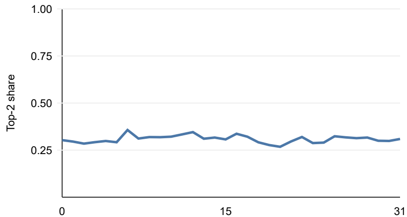
Top-2 expert share across layers
