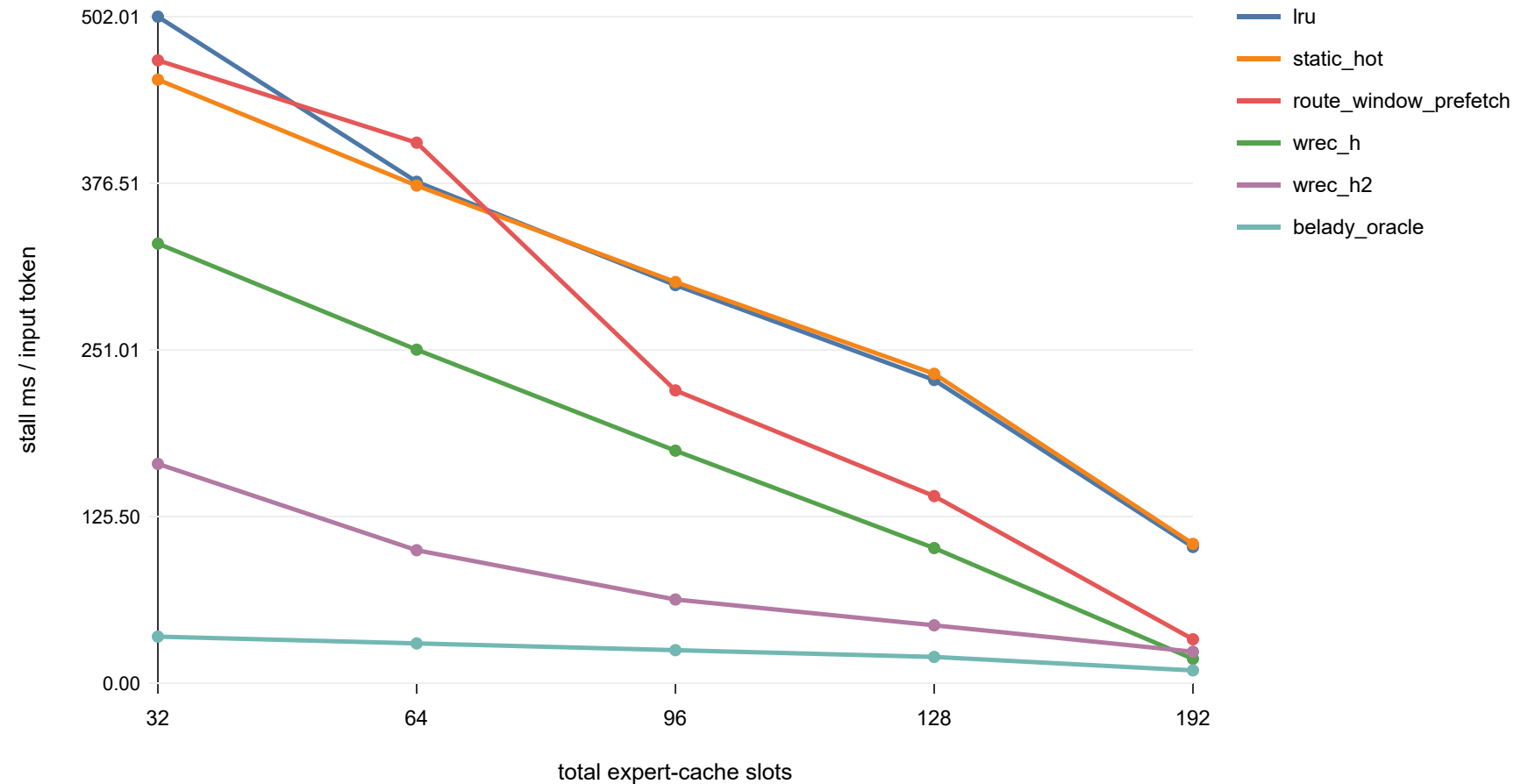
Stall Proxy vs Total Expert-Cache Budget
