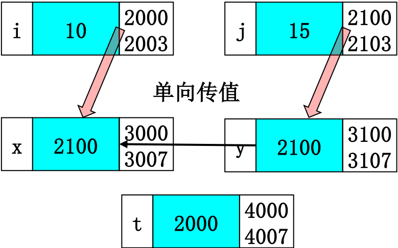
图三 x = y;
