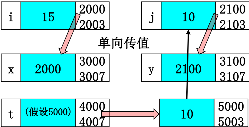
图四 *y = *t;
