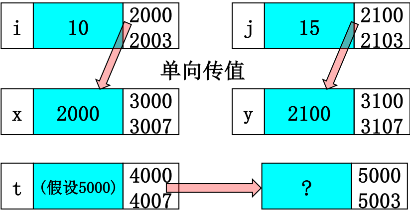
图三 *x = *y;
