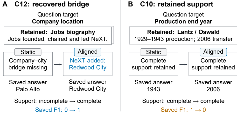
Figure 1: Two observed development examples motivating separate evaluation of evidence selection and answer quality. Short source paraphrases show H4 static and search-aligned contexts, not complete prompts or verbatim quotations. In inspected case C12 (HotpotQA, seed 2026), a recovered company-to-city bridge accompanies increased saved F1. In C10 (MuSiQue, seed 1729), complete annotated support is retained, but the answer changes from the production endpoint to a rights-transfer year present in both contexts. Arrows mark observed selection transitions. These illustrative cases neither estimate prevalence nor establish causality.
