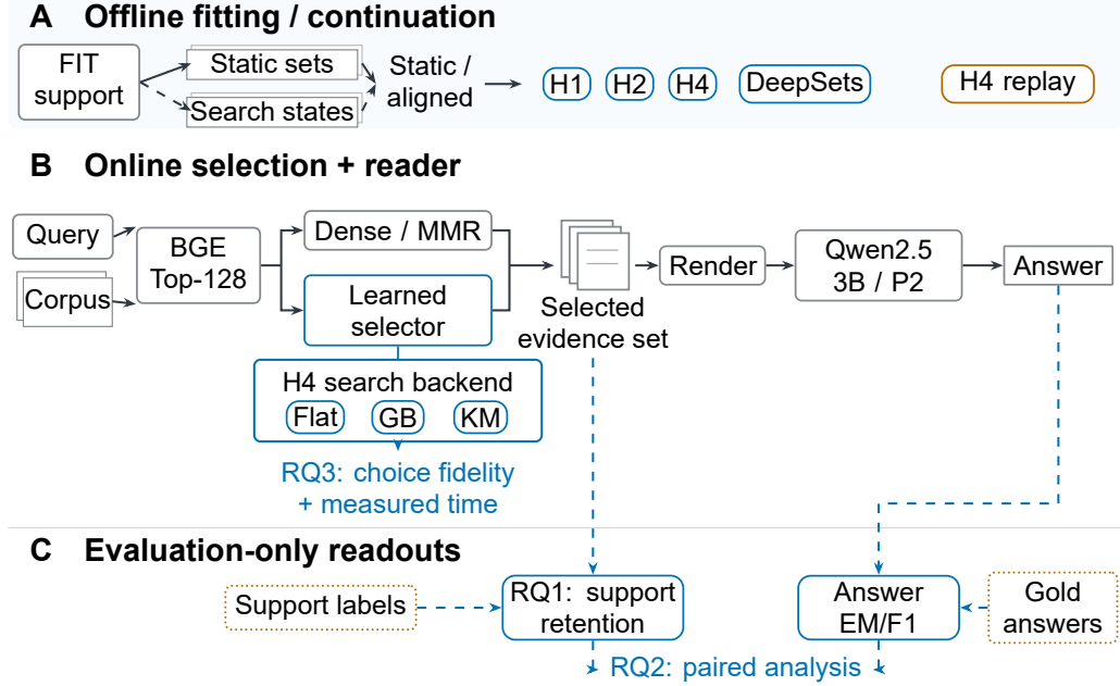
Figure 2: Study design and evaluation interfaces. H1/H2/H4/DeepSets have separately trained parameters; static and search-generated FIT sets supply support supervision, not reader-answer reward. H4 replay matches update counts; supplied-set discrimination is a training diagnostic. With BGE frozen, all methods share the FP16 Qwen2.5-3B/P2 reader, 1,024-token serialized-input ceiling and BGE display order; only learned selectors are limited to six whole paragraphs. Feasible Dense-K6 remains eligible for their final choice. Flat, granular-ball (GB), and k-means (KM) are alternative implementations of the same H4 conditional score, not semantic-relation models or promised accelerators. RQ3 measures fidelity and time at this backend. Dashed readouts join selected support and answers in RQ2; labels never enter deployment inputs. Initial TUNE includes QA; later DEV-SELECT excludes QA. Readouts do not imply online feedback or causality.
