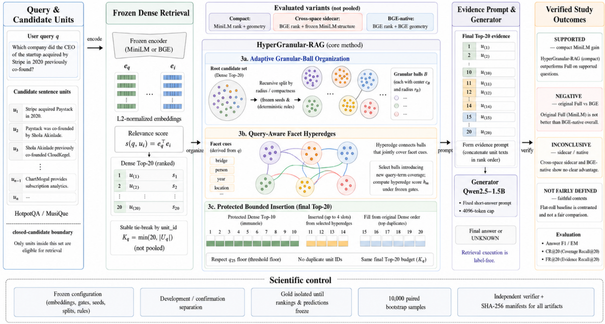
Figure 1: Verified HyperGranular-RAG workflow and study boundaries. Candidate units are ranked by a frozen dense retriever, organized into adaptive granular balls, connected through query-aware facet hyperedges, and inserted under a protected, bounded Top- k policy before frozen answer generation. Compact, cross-space sidecar, and BGE-native variants are evaluated separately rather than pooled. The right column distinguishes supported, negative, inconclusive, and not-fairly-defined outcomes, while the bottom row summarizes the scientific controls applied to the verified experiments.
