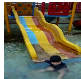
Future I_{t+k}
