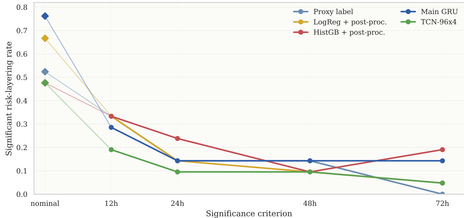
BTCUSDT: significance contracts as block length grows
