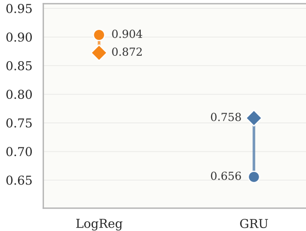
Balanced accuracy
