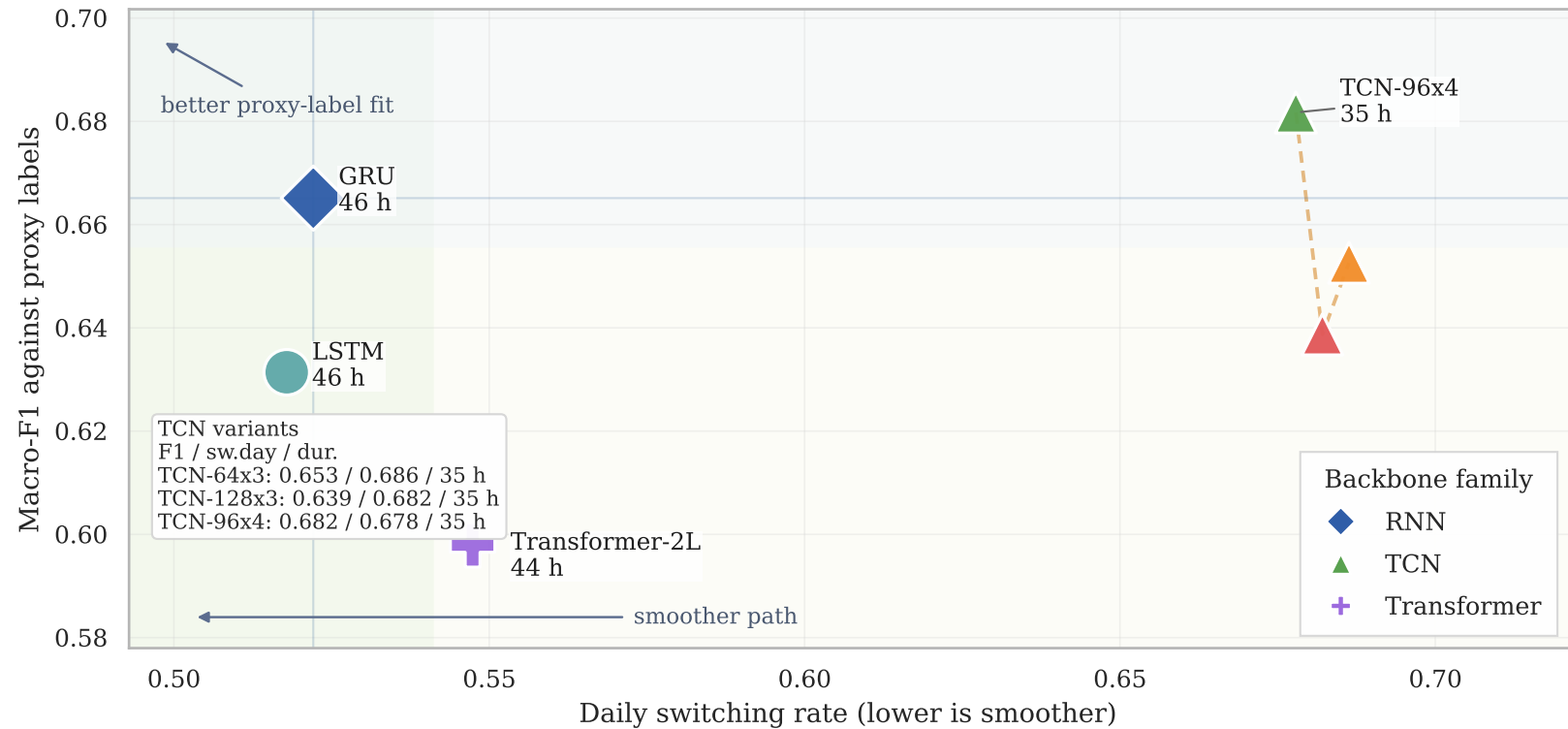
BTCUSDT temporal-backbone tradeoff
