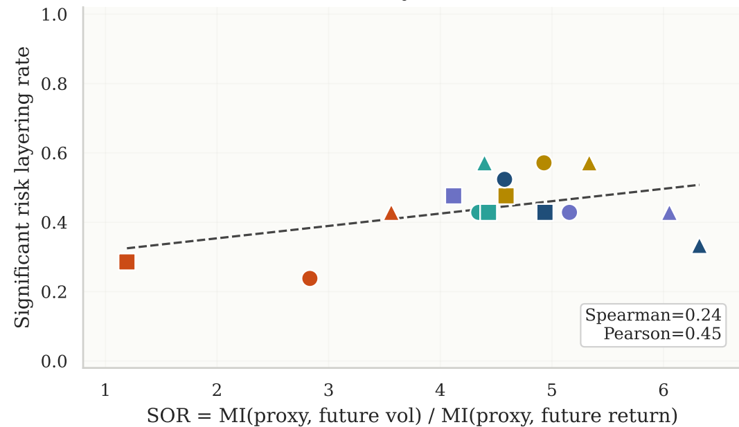
Proxy label
