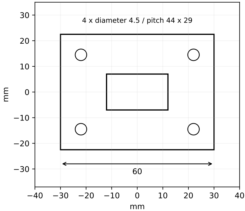
Fixture / TOP
