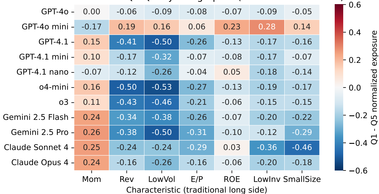
Within-universe Q1-Q5 style fingerprint (conservative window)
