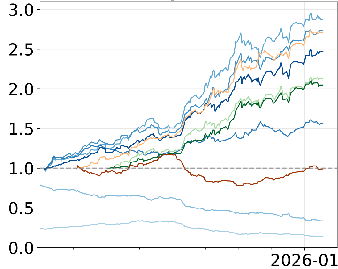
Sharpe Mode
