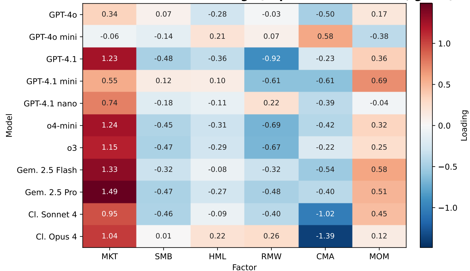
Conservative-window FF6 loadings (expected-return mode, gross)
