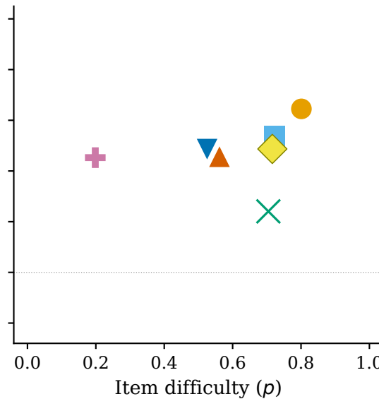
Type centroids
